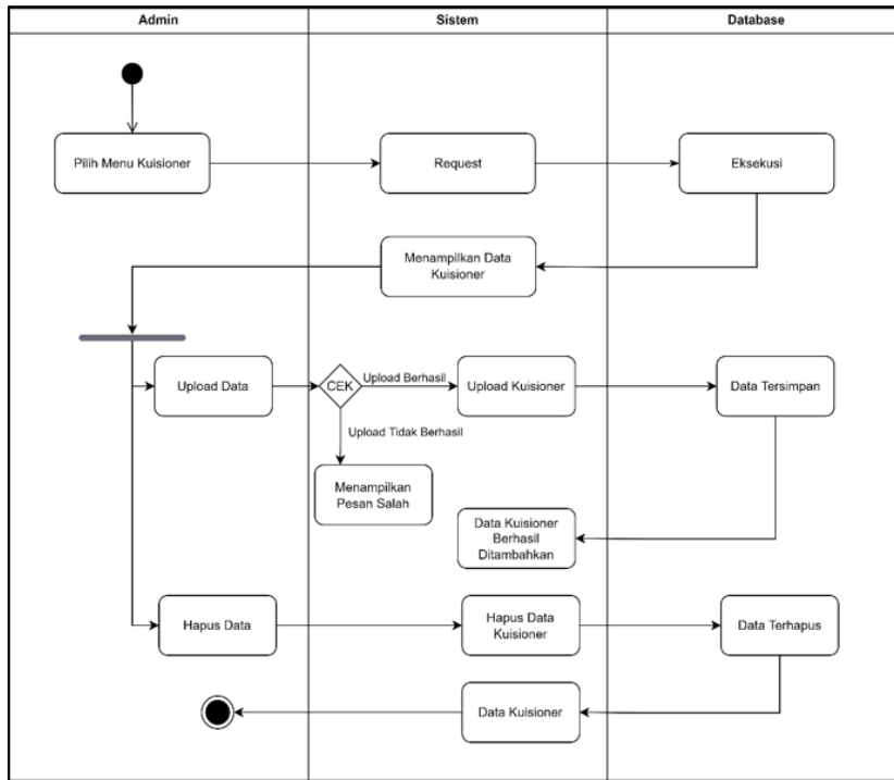
Fig 3. Questionnaire activity diagram.
