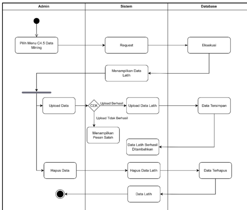
Fig 4. Data mining activity diagram.
