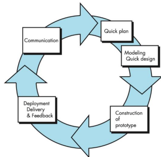
Fig 1. Prototyping model approach
